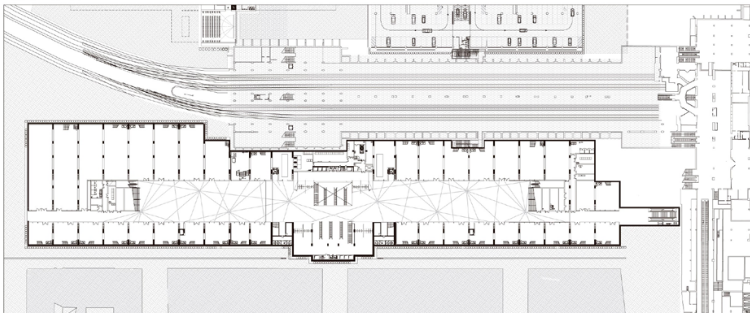
Planta +4.5m Floor +4.5m
